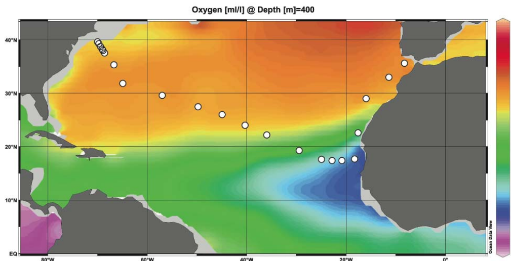
Figure 10: Station locations along the US GEOTRACES North Atlantic cruise track plotted on a map of dissolved oxygen at 400 m, approximately the depth of lowest oxygen concentration (see also Figure 11).
