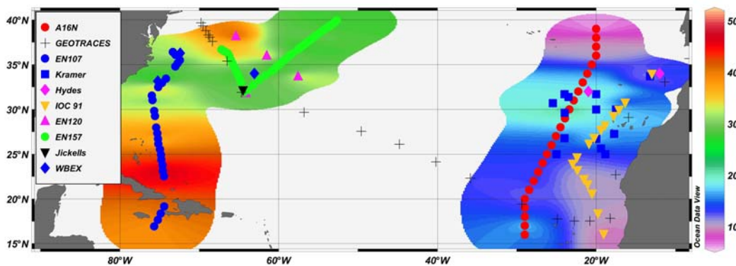
Figure 8: Surface Al concentrations (nM). Modified from a figure in Measures et al. (2008) Proposed stations are shown by “+” symbols.
