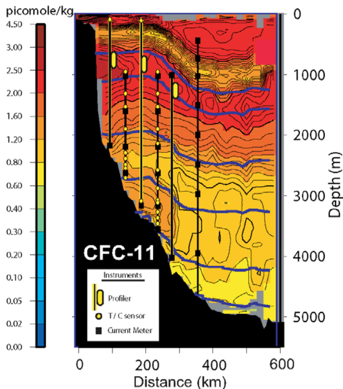
Figure 2: Section plot along Line W of contoured concentrations of CFC-11, an anthropogenic contaminant introduced mainly during the latter half of the 20th century and incorporated into deepwater via gas exchange within regions of deepwater formation. The section plot also depicts the locations of moored instruments that are maintained by the repeat hydrography program. Station locations along the NW portion of the cruise track shown in Figure 1 coincide with the mooring locations shown here. Figure courtesy of John Toole.
