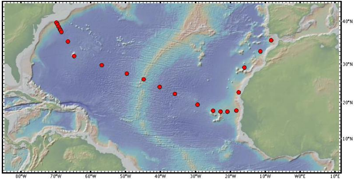
Figure 1: Station locations along the US GEOTRACES North Atlantic cruise track. Red dots represent stations where full water column TEI sampling is anticipated. Additional sampling of surface waters, and shallow (e.g., to 1000 m) hydrocasts, will be employed to provide greater spatial resolution in selected areas of the cruise track. This map was produced using GeoMapApp: http://www.geomapapp.org/ .
