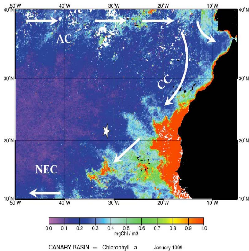
Figure 9: Phytoplankton biomass in January 1999 estimated using the SeaWiFS sensor illustrates the strong gradients in biological productivity and biogenic particle flux that are anticipated to occur along the eastern portion of the US GEOTRACES section. The white arrows indicate offshore transport by the Canary Current, which distributes the biogenic particles generated within the productive upwelling system over a larger area than would occur in a simple linear coastal upwelling regime. Reprinted from Deep Sea Research Part II: Topical Studies in Oceanography , Vol. 48/Iss. 10, I. Dadou, F. Lamy, C. Rabouille, D. Ruiz-Pino, V. Andersen, M. Bianchi, V. Garçon, An integrated biological pump model from the euphotic zone to the sediment: a 1-D application in the Northeast tropical Atlantic. JGOFS Research in the North Atlantic Ocean: A Decade of Research, Synthesis and modelling , Pages 2345-2381, Copyright (2001), with permission from Elsevier. http://www.sciencedirect.com/science/journal/09670645 .
