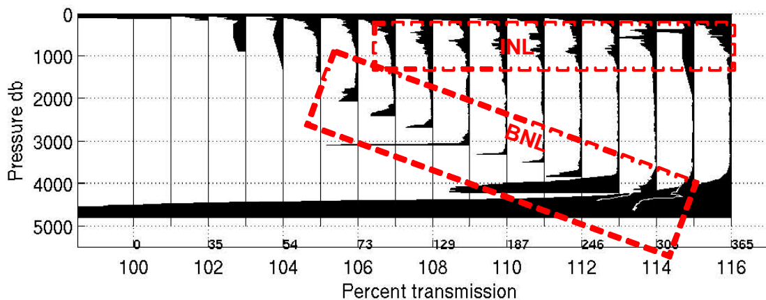
Figure 6: Transmissometry profiles along Line W, depicting both intermediate and benthic nepheloid layers extending a large distance away from the shelf. Small numbers just above the x-axis labels are distance in kilometers from a station just landward of the shelf break. Figure courtesy of John Toole
