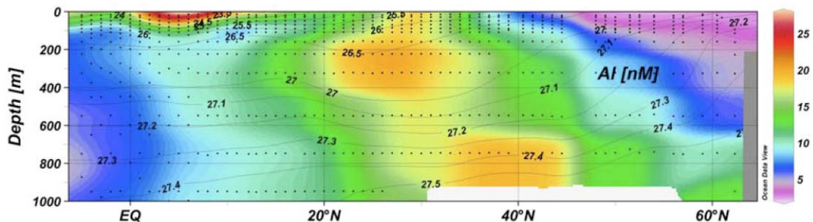
Figure 3. Dissolved Al concentrations (nM) along the CLIVAR A16 section in the eastern N Atlantic Ocean. High concentrations at the surface between the equator and 10°N reflect dissolution from recent dust deposition. The elevated concentrations between 200 and 400 m (20°N to 35°N) are associated with Mode Water advection, while the elevated concentrations between 800 and 1000 m (30° to 45°N) are associated with high salinity water from the Mediterranean Sea. From Measures et al., (2008).
