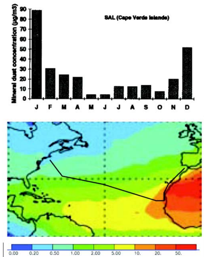
Figure 7: Seasonality (upper panel, from Chiapello et al, 1995; reproduced with permission from the American Geophysical Union) and distribution of dust deposition (lower panel, in \text{g m}^{-2} \text{y}^{-1} , from Jickells et al, 2005; Reproduced with permission from AAAS, http://www.sciencemag.org .) in the North Atlantic. Proposed section shown in lower panel as a black line.
