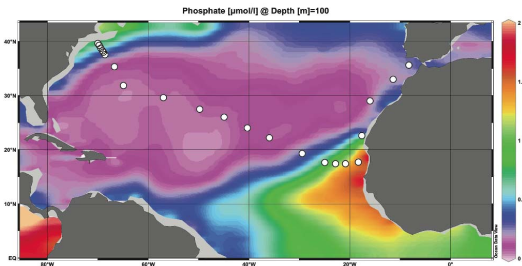
Figure 5: Station locations plotted on a map of dissolved phosphate at 100 m. Downwelling of nutrient-depleted surface waters maintains low nutrient concentrations at 100 m throughout the gyre. Higher concentrations near the margins reflect upwelling and/or seasonal deepening of the mixed layer, both of which bring nutrients into the euphotic zone.
