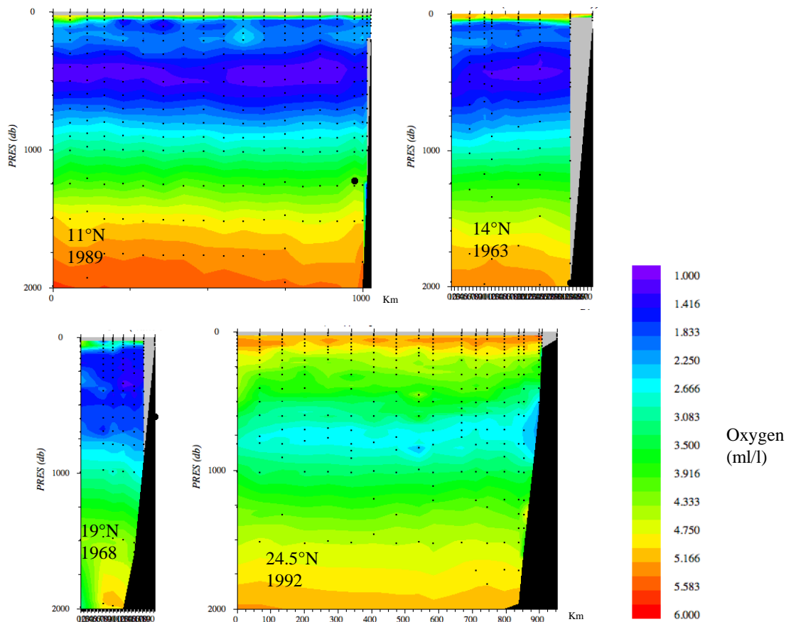
Figure 11: Zonal sections of oxygen concentration in the northeastern Atlantic crossing the oxygen minimum zone to the African continental shelf. Minimum oxygen concentrations occur between 400 and 500 m. Figure compiled by Bill Smethie. (see also Figure 10).
