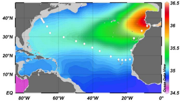
Salinity [psu] @ Depth [m]=1200
