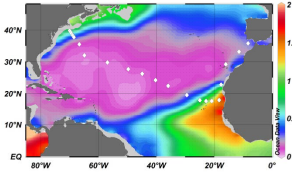
Phosphate [ \mu\text{mol/l} ] @ Depth [m]=100
