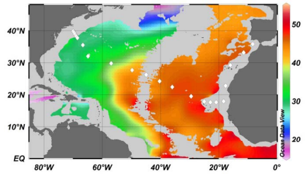
Silicate [ \mu\text{mol/l} ] @ Depth [m]=4000
